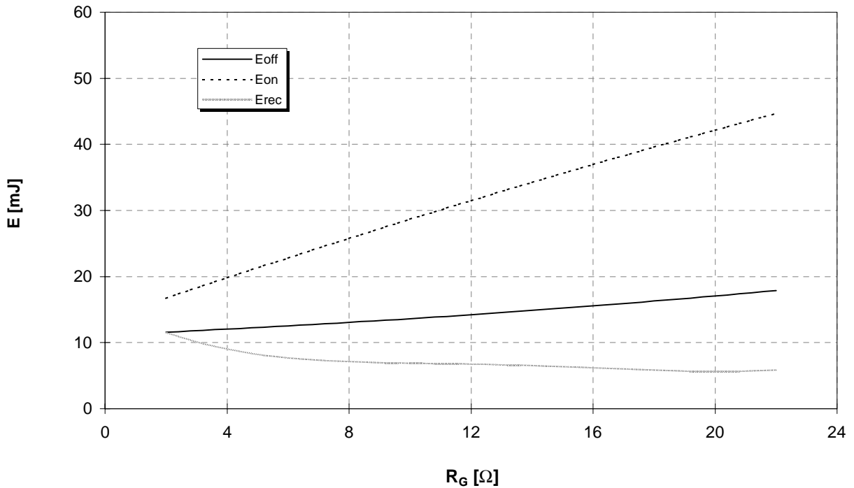
Schaltverluste (typisch) E_{on} = f(R_G), E_{off} = f(R_G), E_{rec} = f(R_G) Switching losses (typical) I_C = 150A, V_{CE} = 600V, T_j = 125^\circ C
