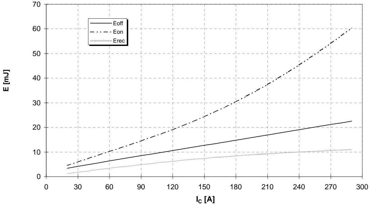
Schaltverluste (typisch) E_{on} = f(I_C), E_{off} = f(I_C), E_{rec} = f(I_C) Switching losses (typical) R_{gon} = R_{goff} = 5,6 \Omega, V_{CE} = 600V, T_j = 125^\circ C
